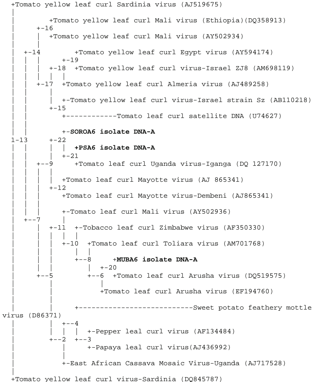
Figure 3: Phylogenetic relationship between the Isolates identified, other Tomato Viruses in Africa and Leaf Curl Viruses Infecting Crops in the Tomato Agro-ecosystem
